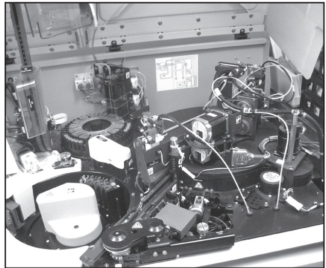
Closed system (above) weighs 750 pounds. Under the hood (right), test tubes move through for analysis. The machine performs up to 400 laboratory tests per hour.
